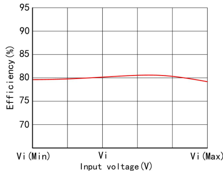
Efficiency/Input voltage diagram
