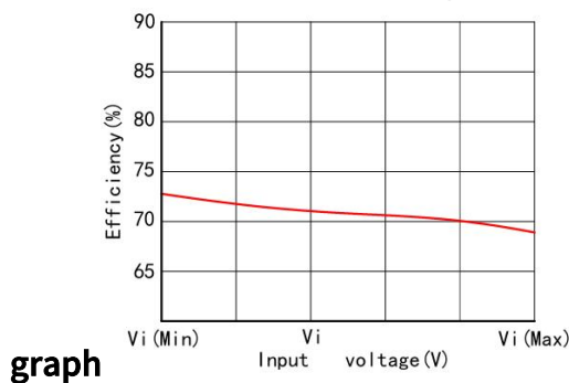
Efficiency/Input voltage
