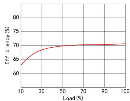
Efficiency/Load graph
