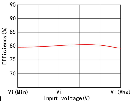
Efficiency/Input voltage
