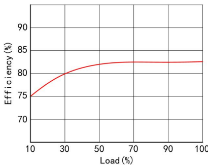
Efficiency/Load graph
